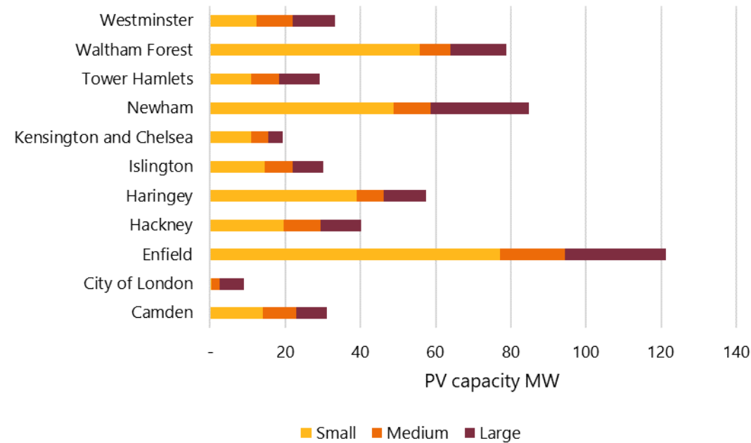
Figure 3—11 PV capacity in 2040 per borough for the Baseline and Network Led scenarios.
