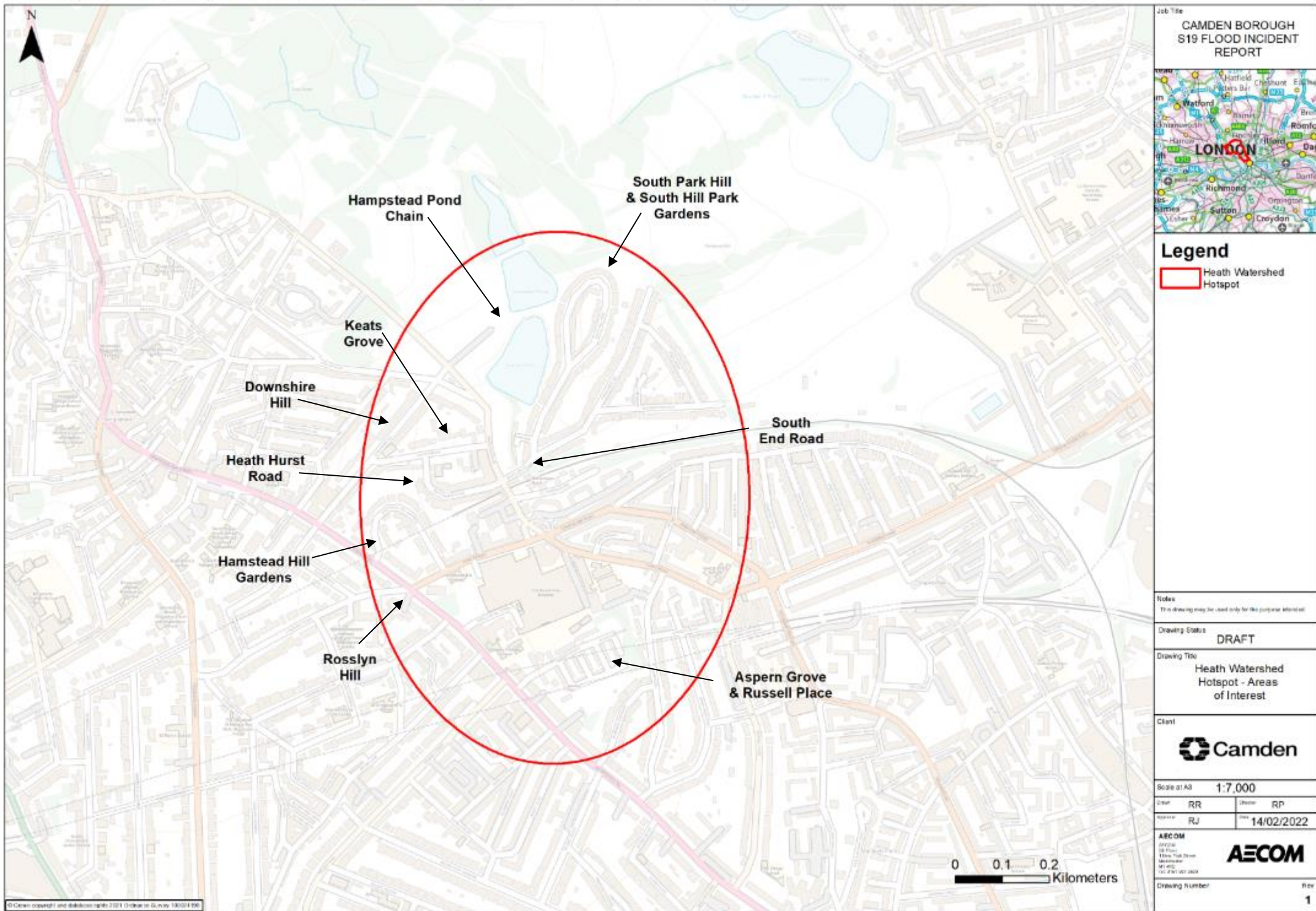
Figure 4-5: Heath Watershed Hotspot
